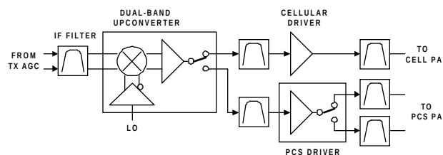
Fig. 1 Block diagram of a dual-band transmitter.
